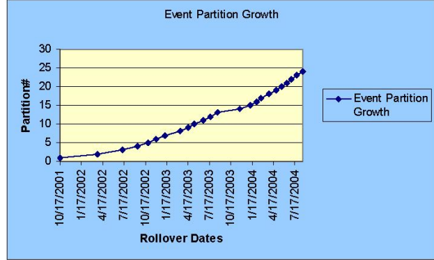
Figure 4 Partition growth for D0 Event table.
