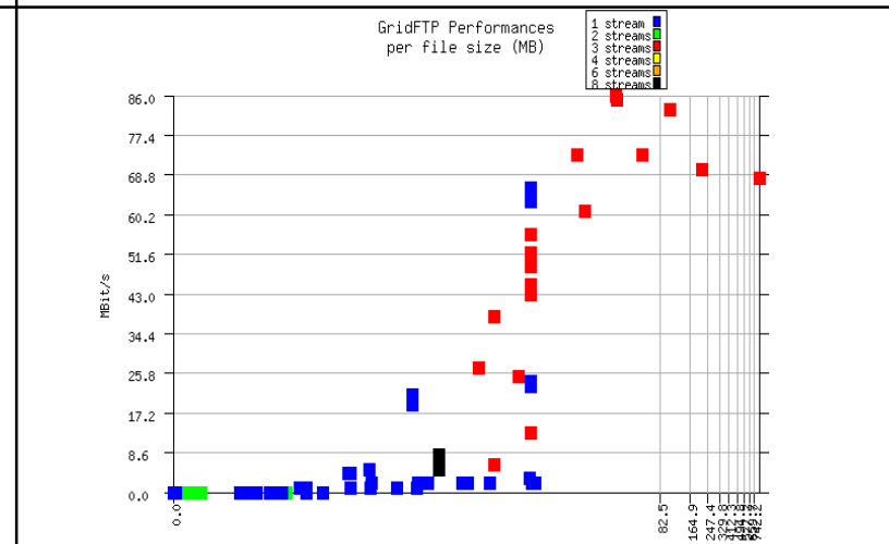
GridFTP performances analysis
