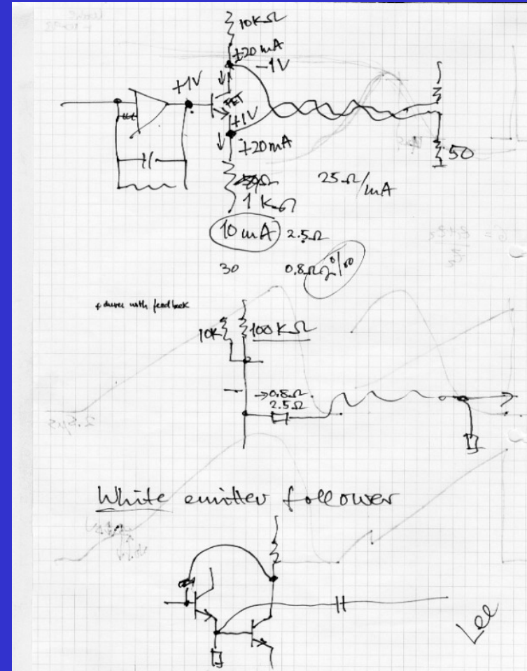
Designing the input stage for the CPD
