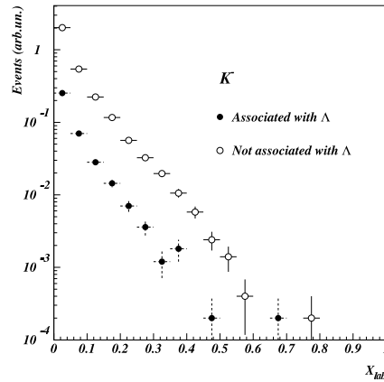
Figure 8. X_{lab} distributions of K^- produced in p–Air collisions at E_0 = 100 GeV. Events where K mesons are associated to \Lambda production are distinguished from the others.
