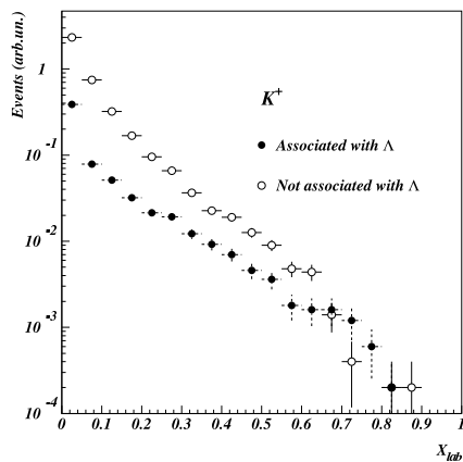
Figure 6. X_{lab} distributions of K^+ produced in p-Air collisions at E_0 = 100 GeV. Events where K mesons are associated to \Lambda production are distinguished from the others.
