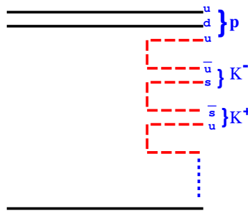
Figure 5. Example where K^+ K^- (or K^0 \bar{K}^0 if d quark replace the u one) are produced, without any associated strange baryon.
