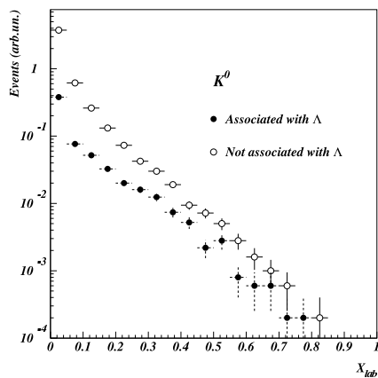
Figure 7. X_{lab} distributions of K^0 produced in p-Air collisions at E_0 = 100 GeV. Events where K mesons are associated to \Lambda production are distinguished from the others.
