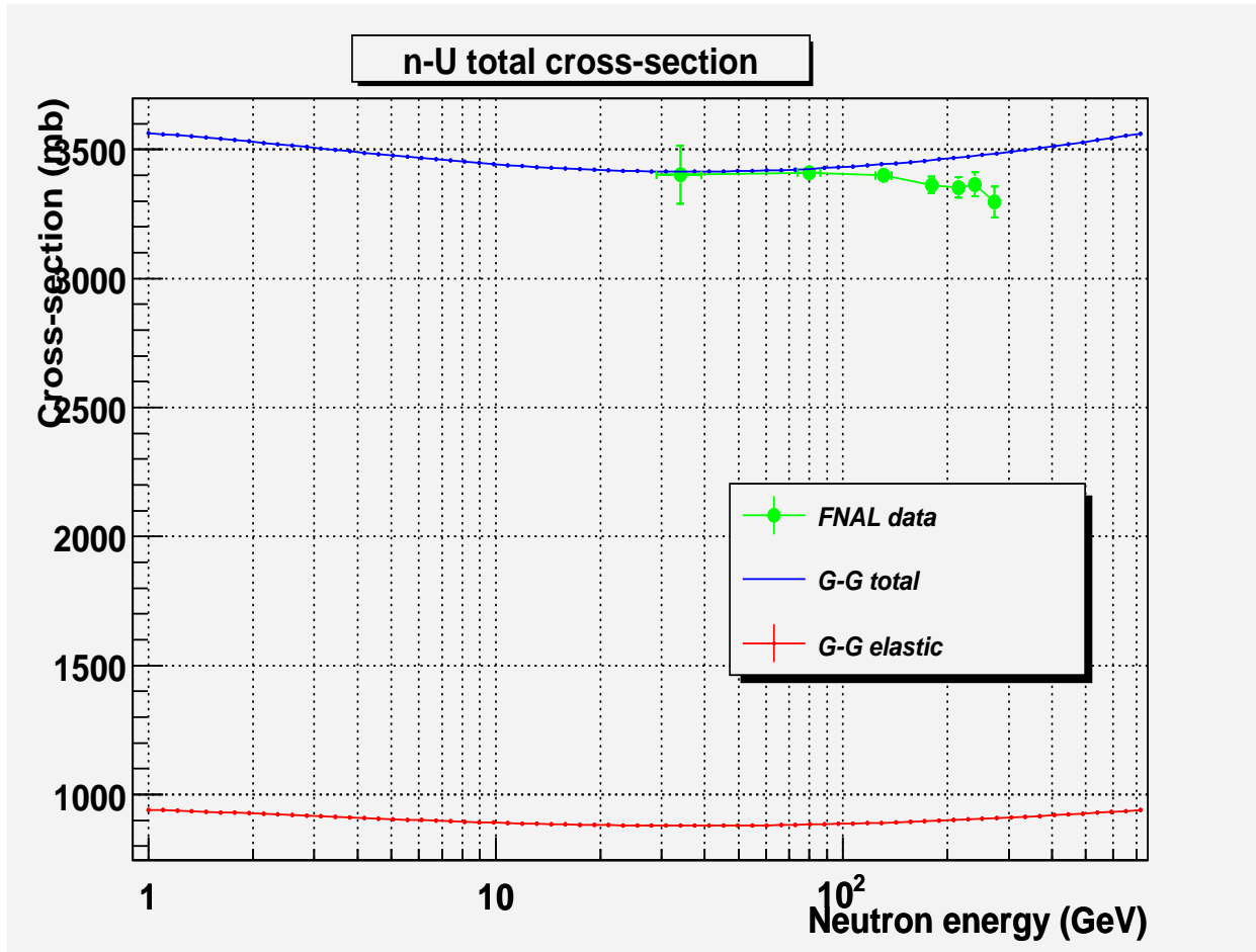
Elastic and total cross sections of neutrons on uranium target versus the neutron energy in the laboratory frame.
