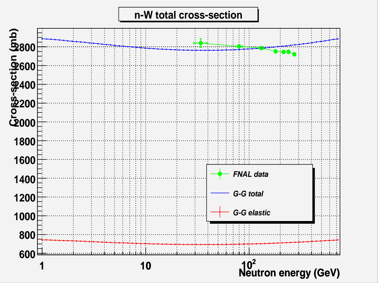
Elastic and total cross sections of neutrons on tungsten target versus the neutron energy in the laboratory frame.
