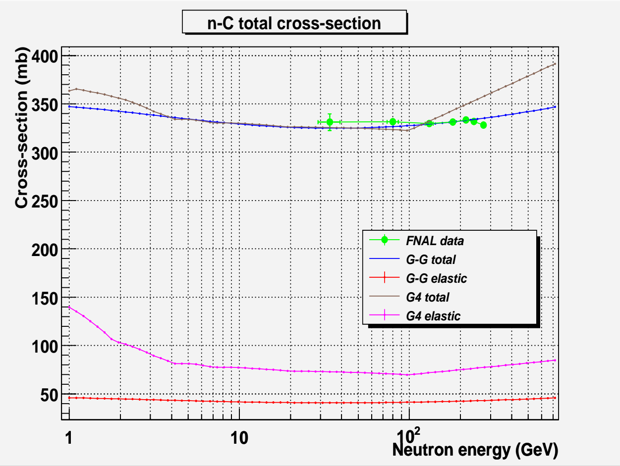
Elastic and total cross sections of neutrons on carbon target versus the neutron energy in the laboratory frame. Geisha (G4) and Glauber-Gribov (GG) models are shown.
