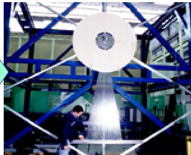
CMS
